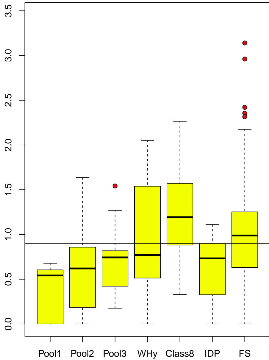
pctF/Unip vs group
