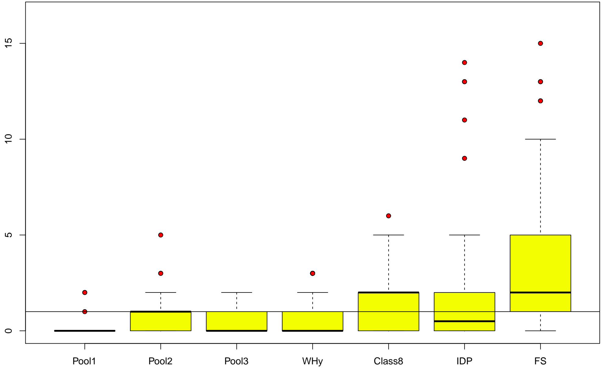
cntW vs group
