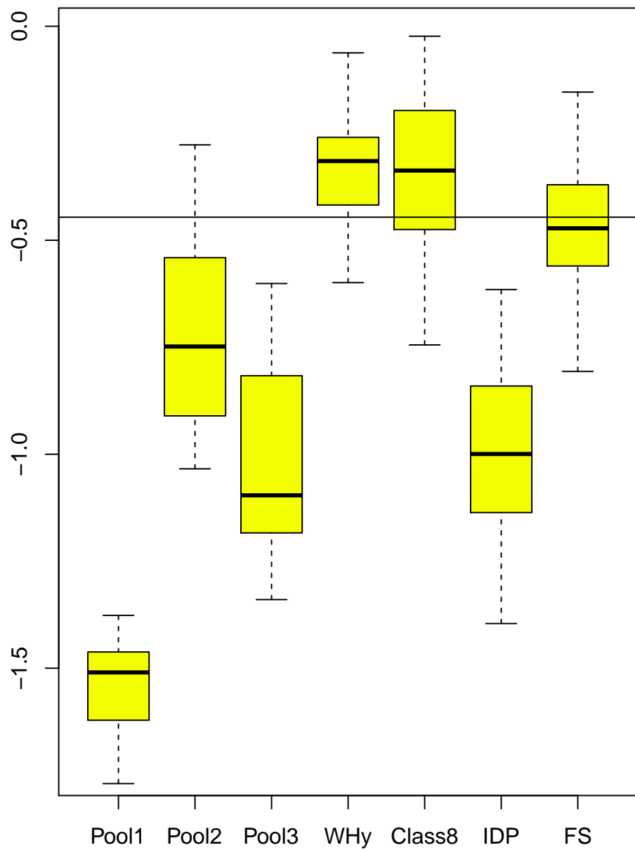
TRANSM vs group
