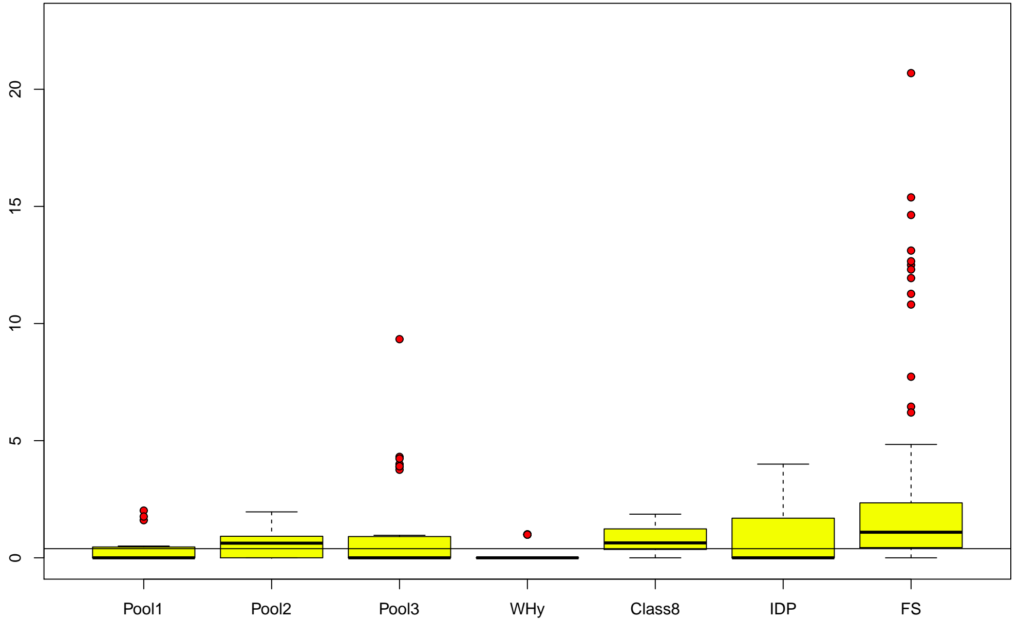
pctC vs group
