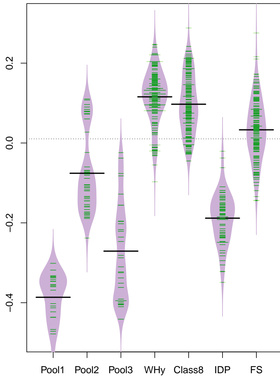
HYDROPHO vs group
