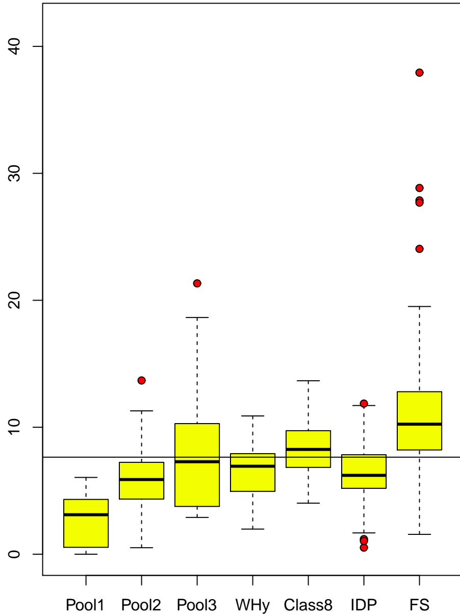
C+F+Y+W vs group
