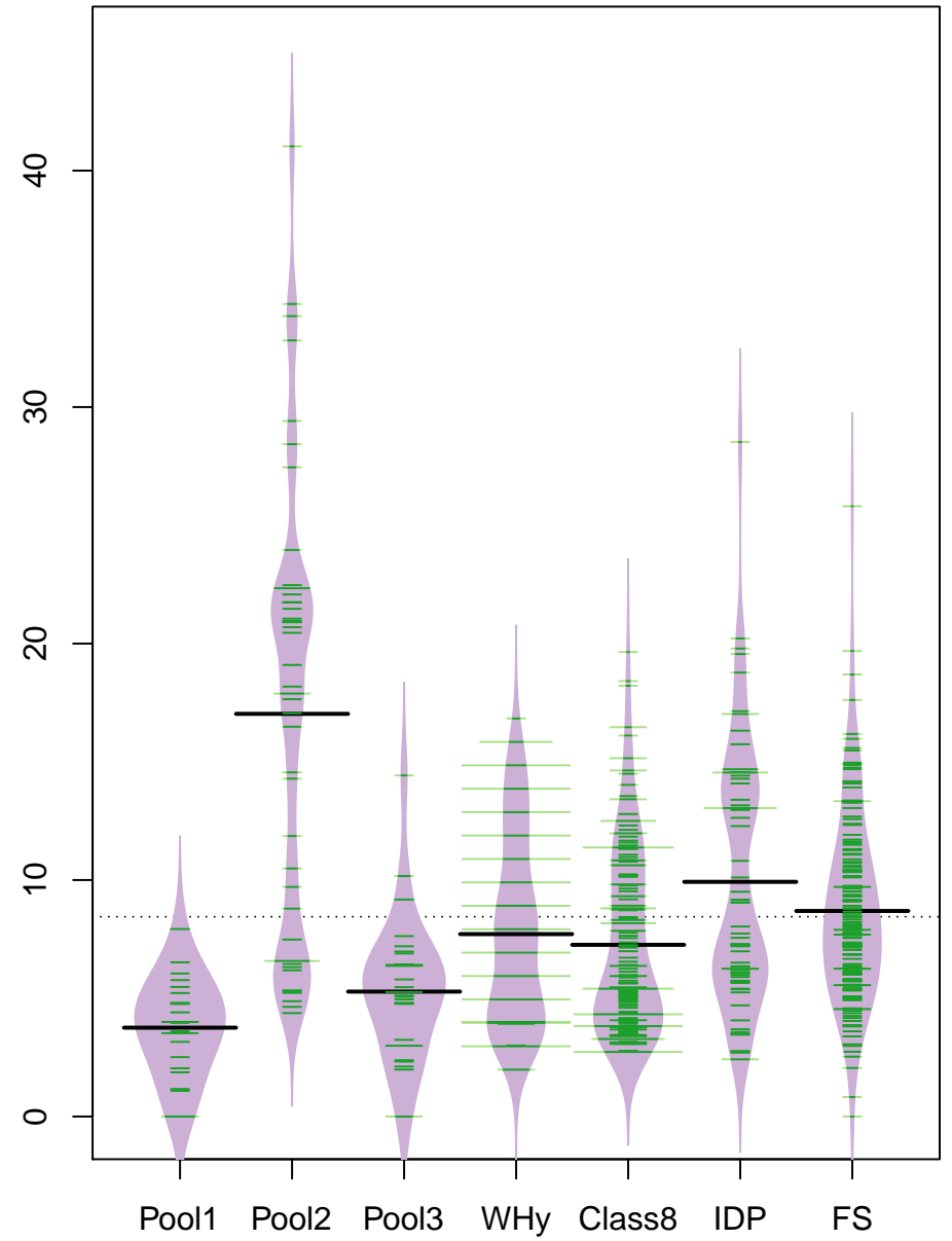
pctA vs group
