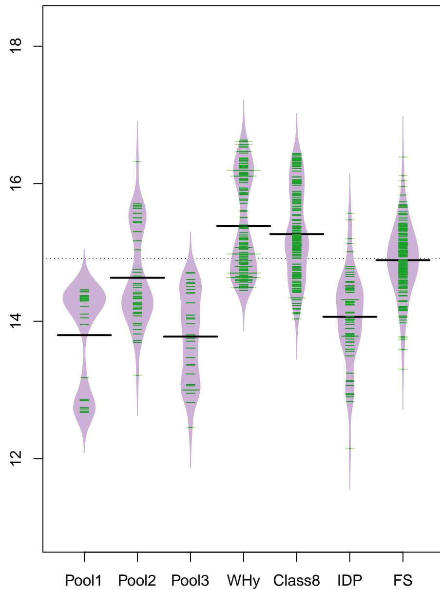
BULKI vs group
