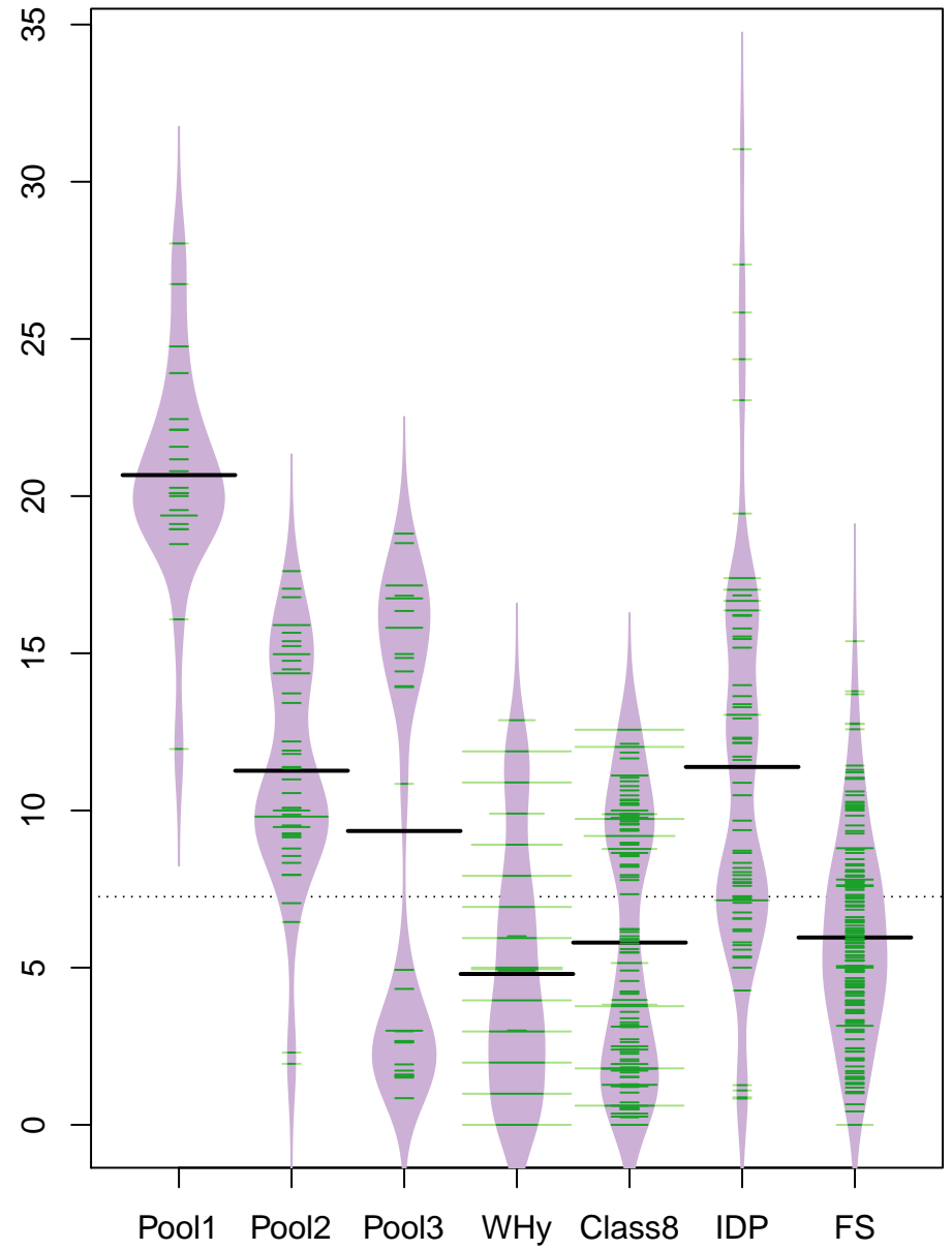
pctK vs group
