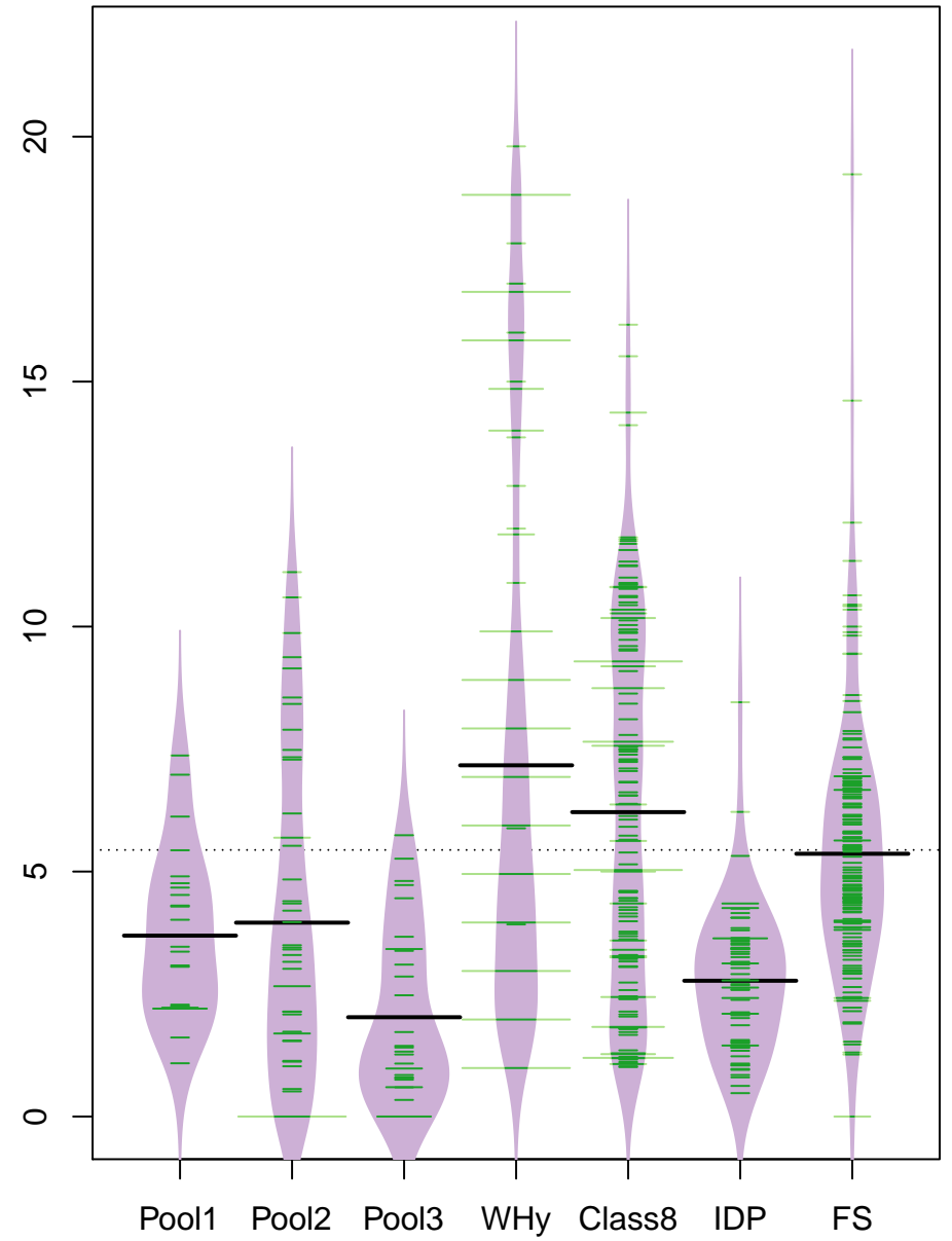
pctl vs group
