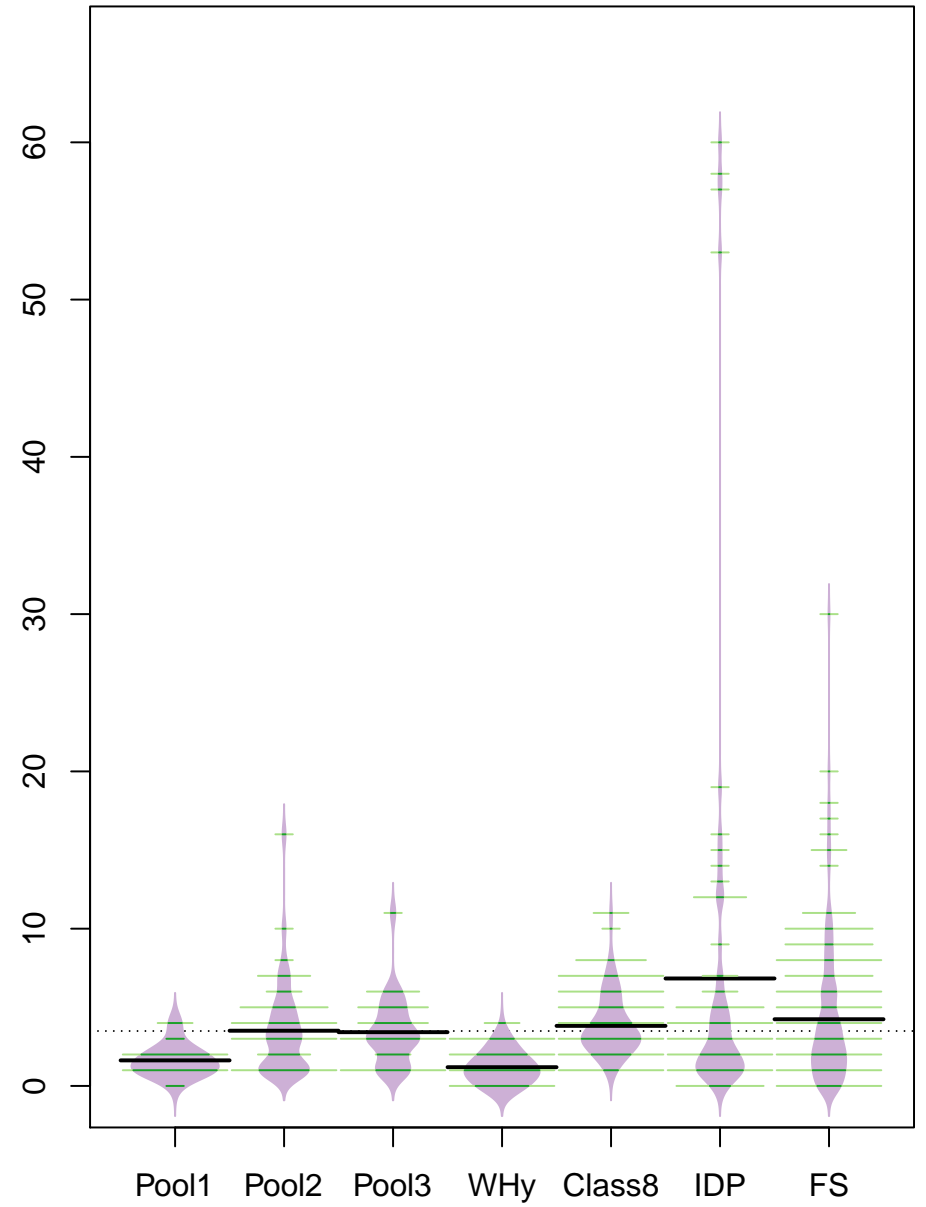
cntM vs group
