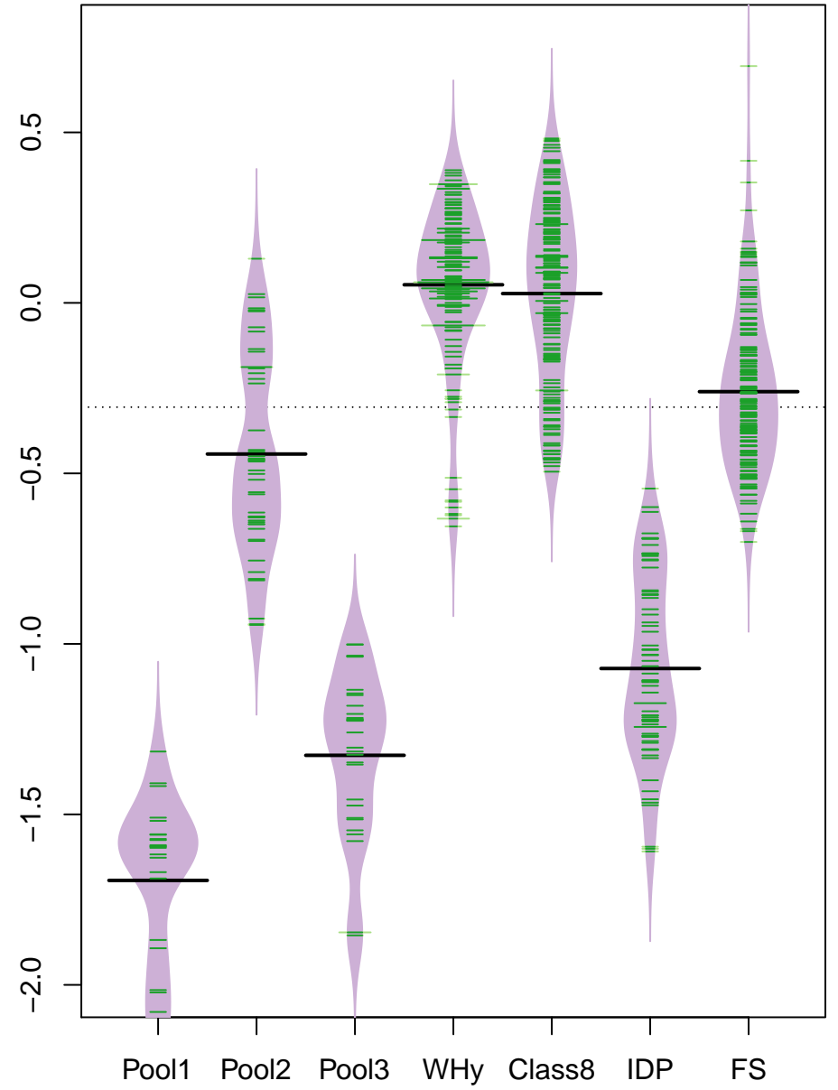
GRAVY vs group
