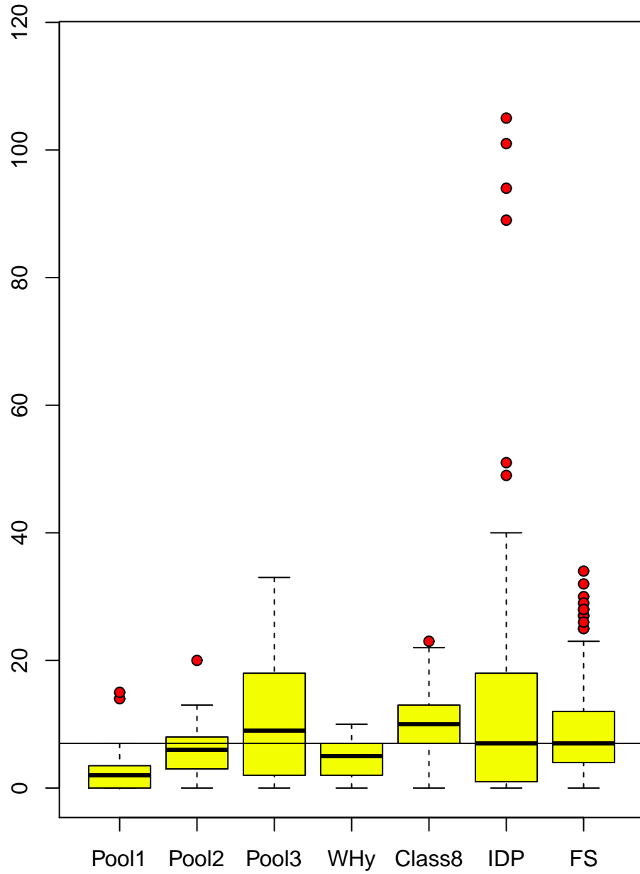
cntR vs group
