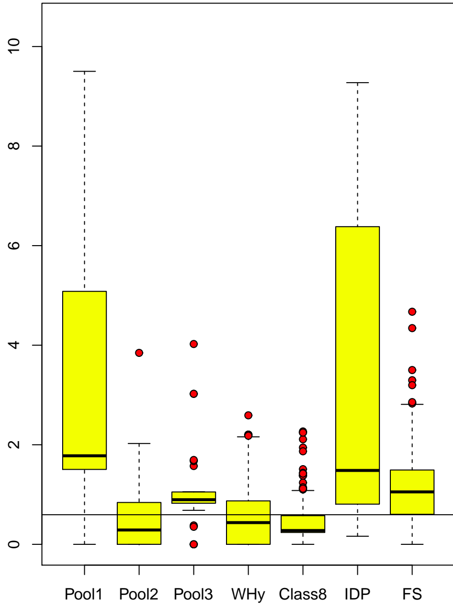
pctH/Unip vs group
