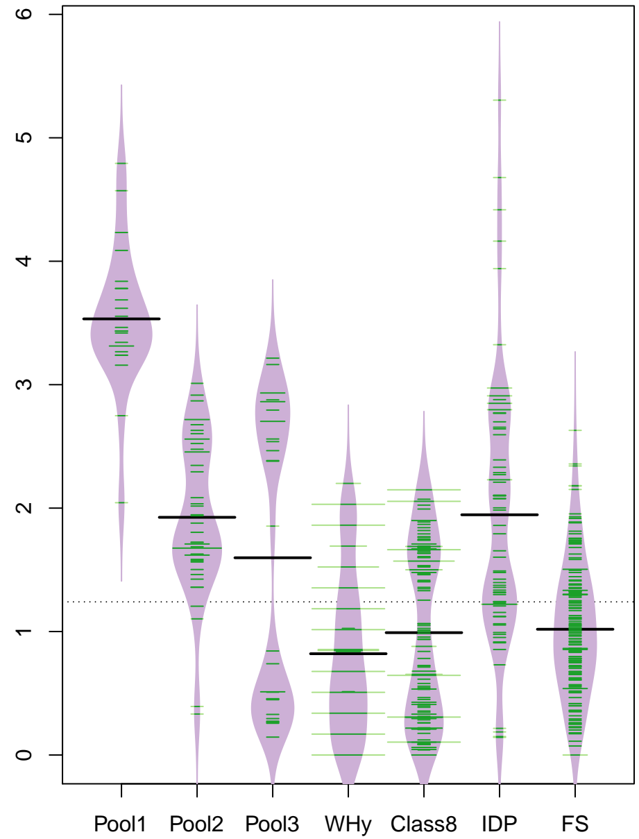
pctK/Unip vs group
