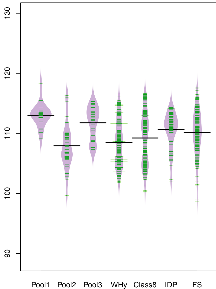
MW/LENGTH vs group
