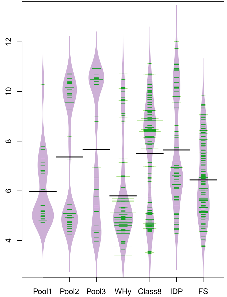
PI vs group
