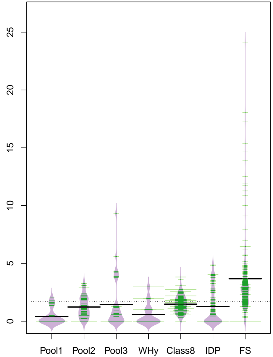
C+W vs group
