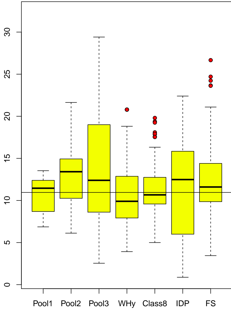
S+T vs group
