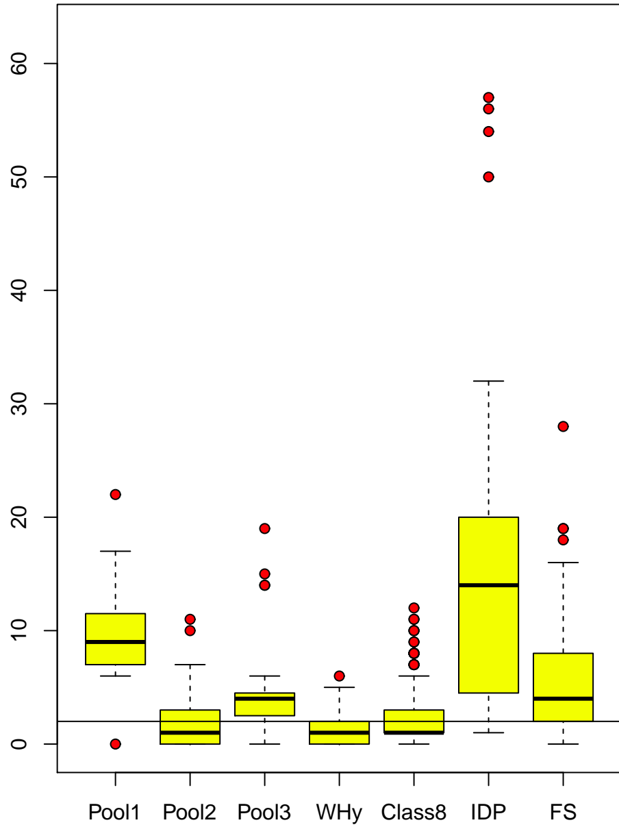
cntH vs group
