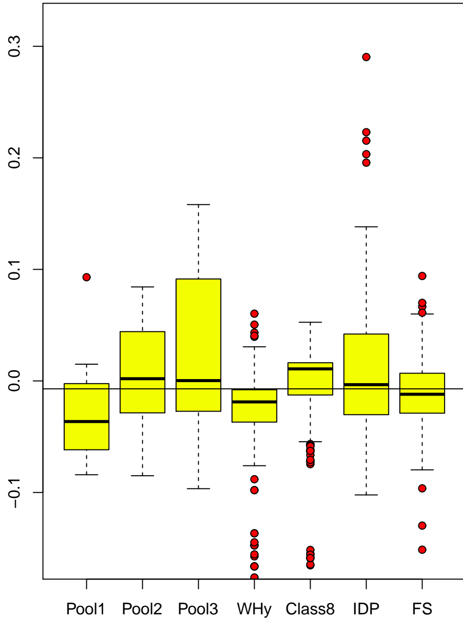
CHARGE vs group
