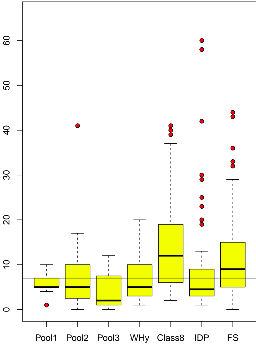
cntl vs group
