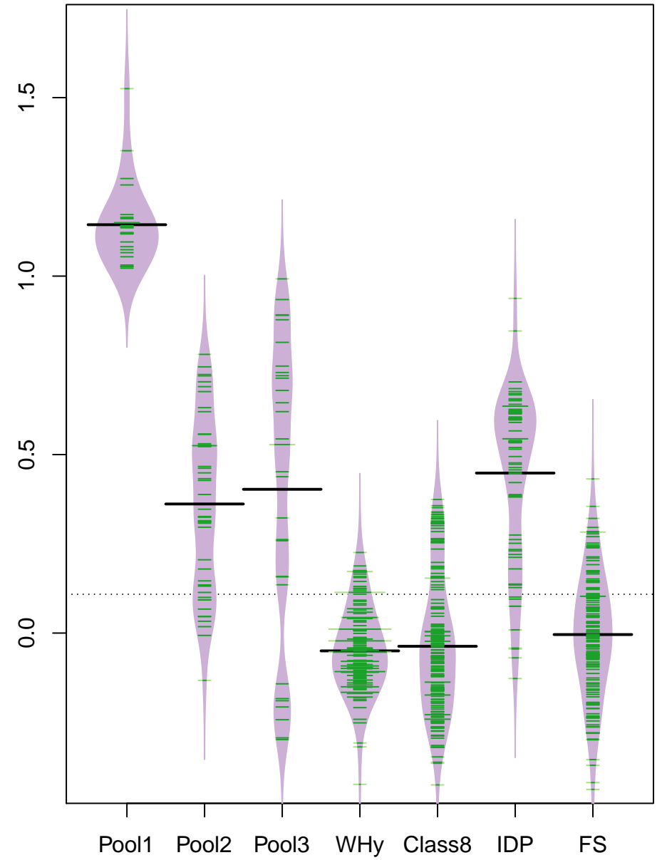
HYDROPHI vs group
