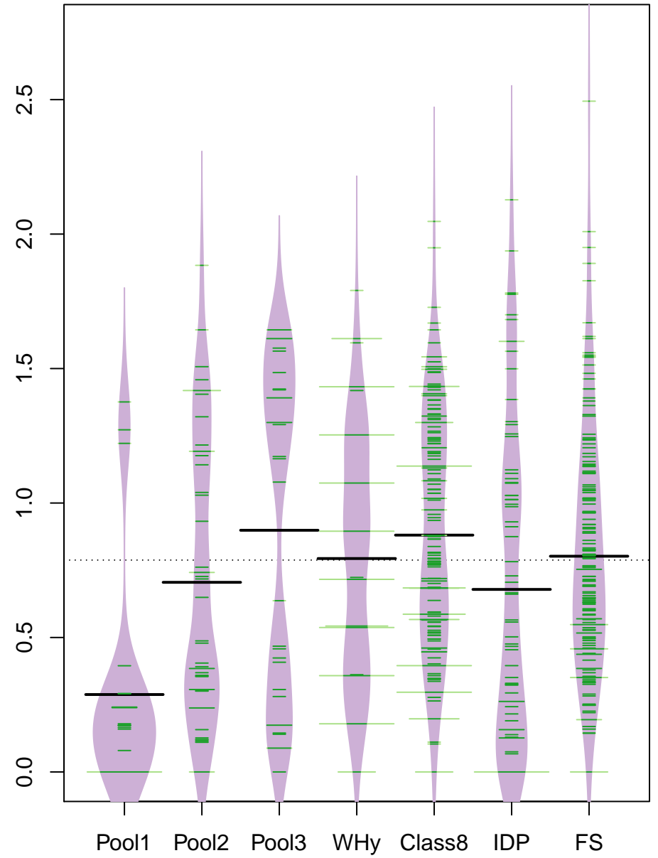
pctR/Unip vs group
