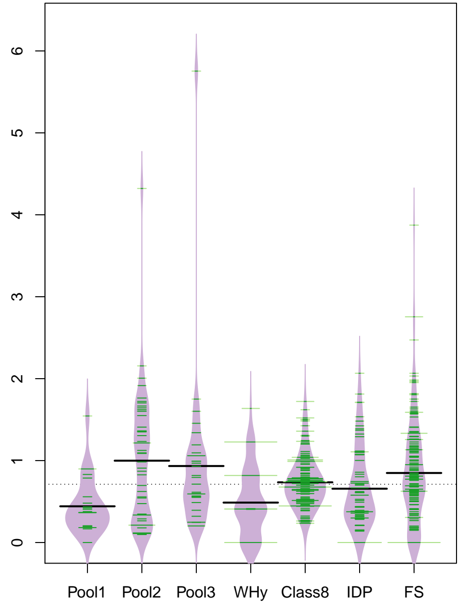
pctM/Unip vs group
