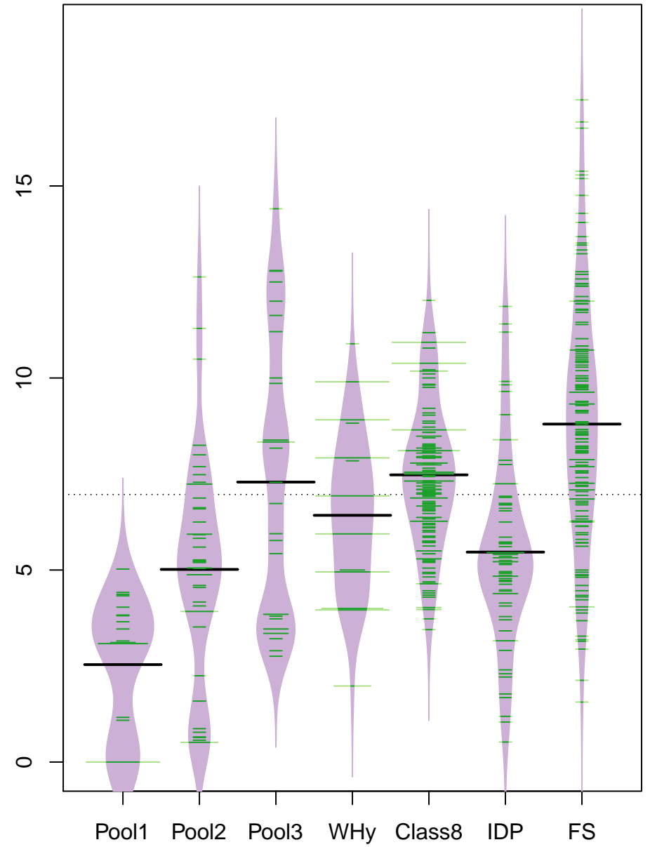
F+W+Y vs group
