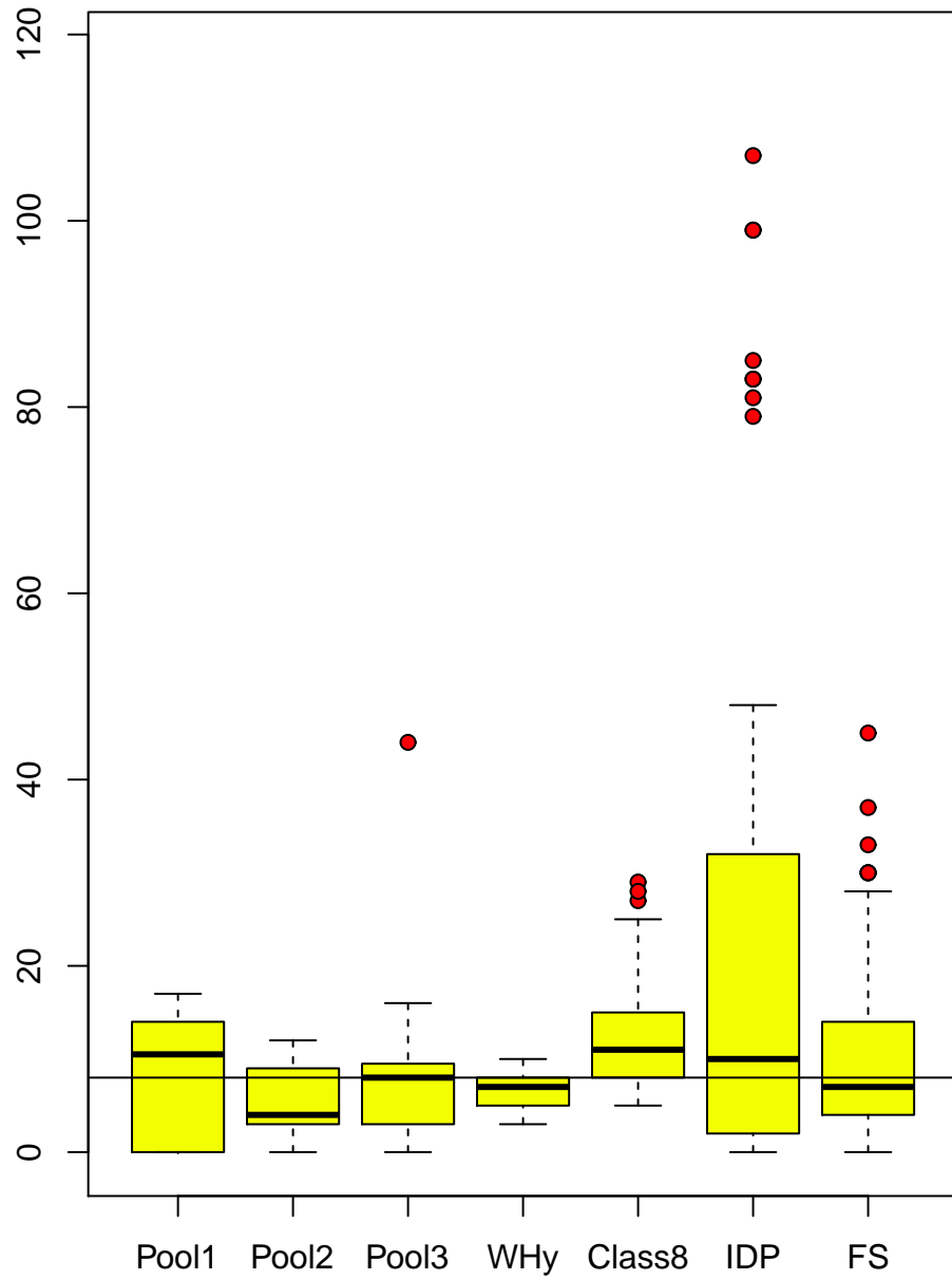
cntP vs group
