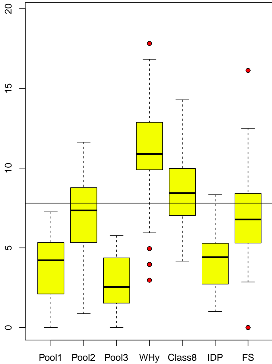
pctV vs group
