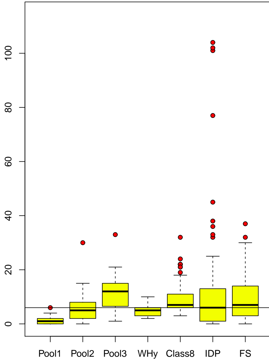
cntN vs group
