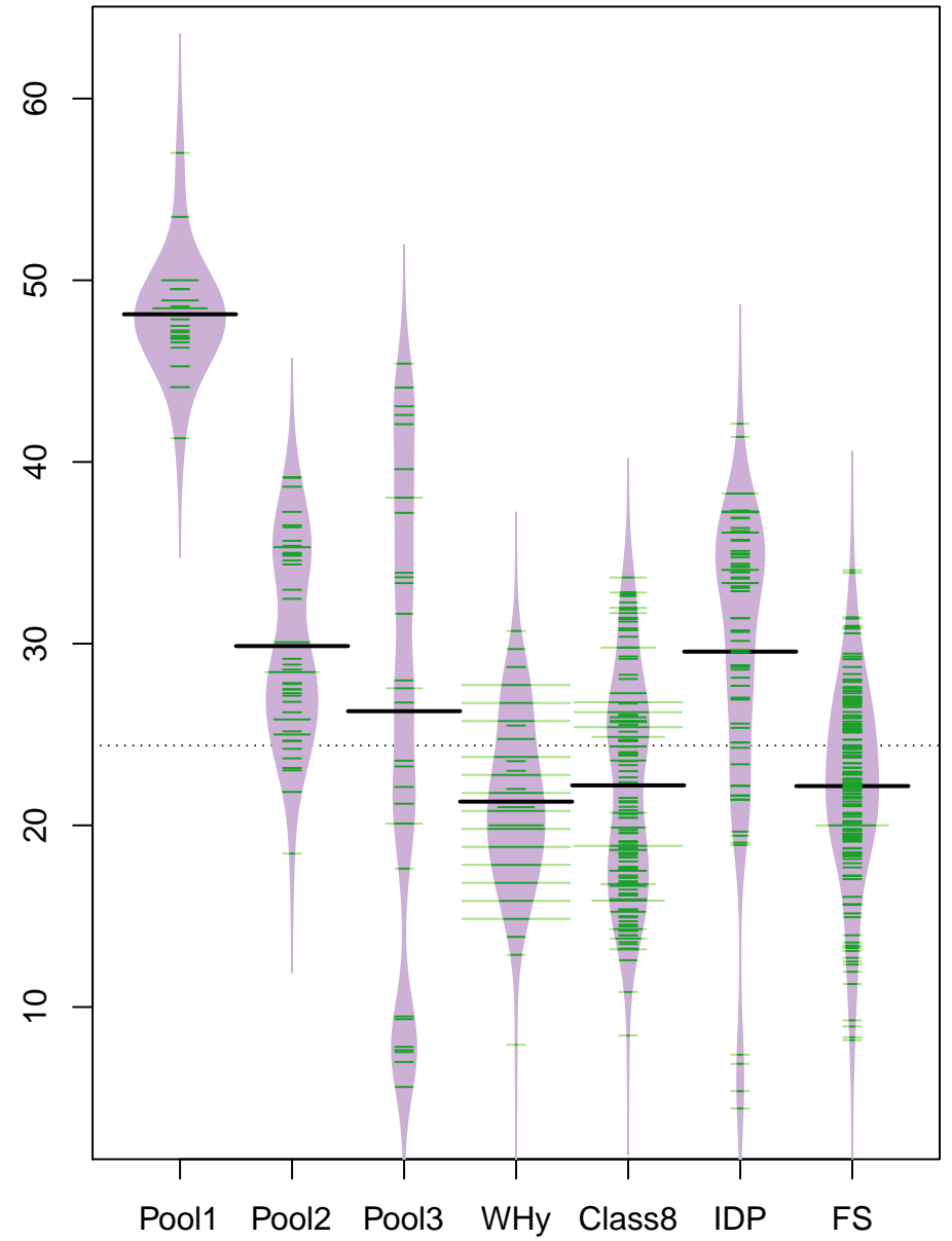
D+E+K+R vs group
