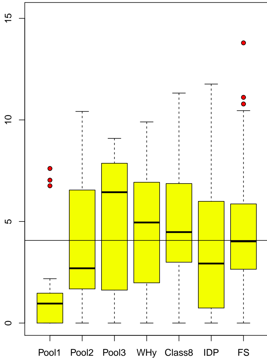
pctR vs group
