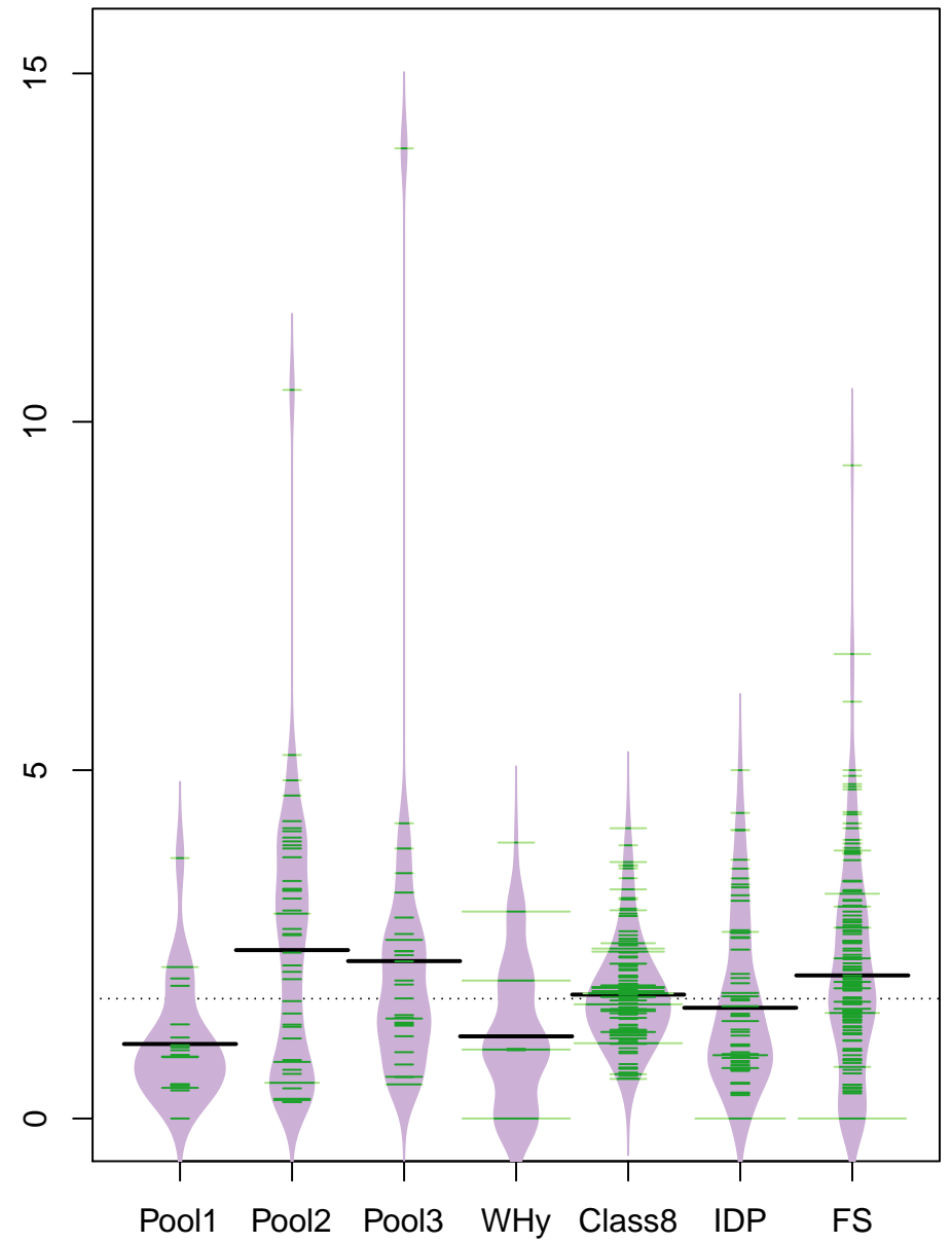
pctM vs group
