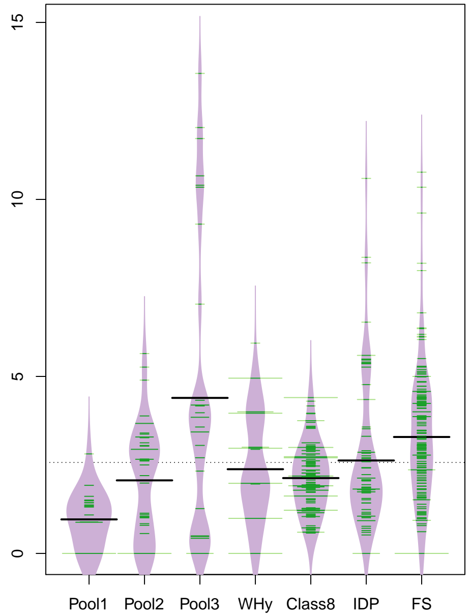
pctY vs group
