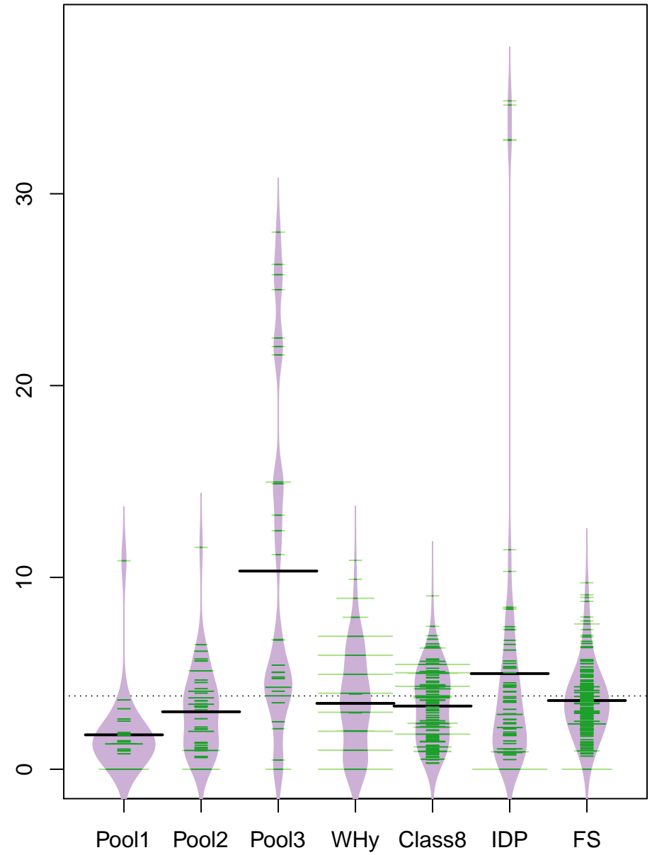
pctQ vs group
