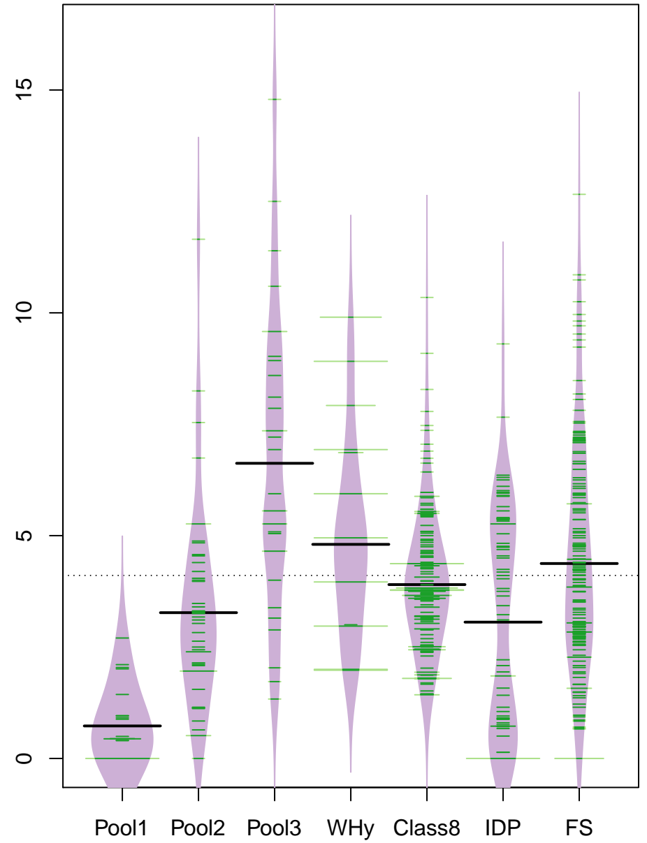
pctN vs group
